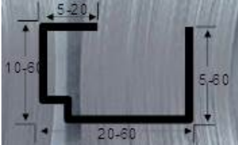
CRACKED CORNER G PROFILE
